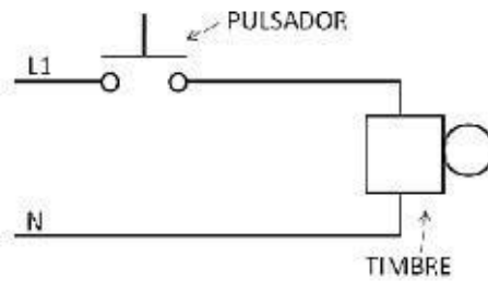
diagrama multifilar
