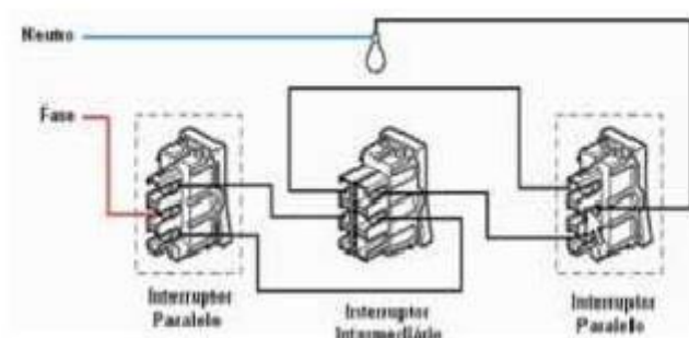
diagrama multifilar
